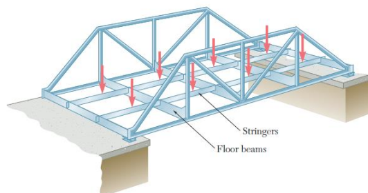
Figura 01 –Treliza Warren
